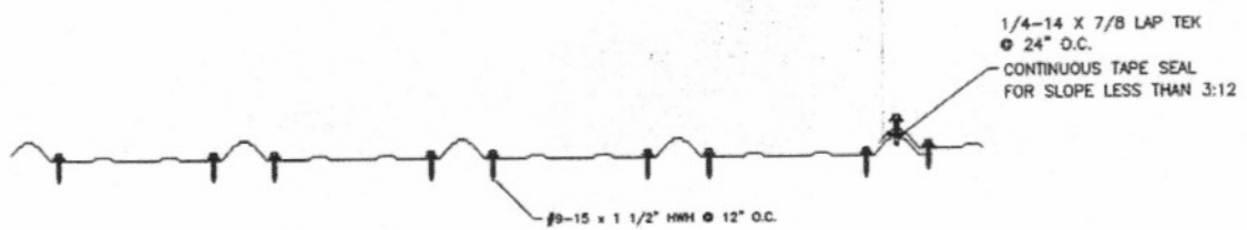
TYPE 2 FASTENER PATTERN
