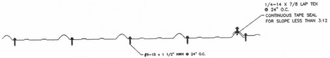
TYPE 1 FASTENER PATTERN
