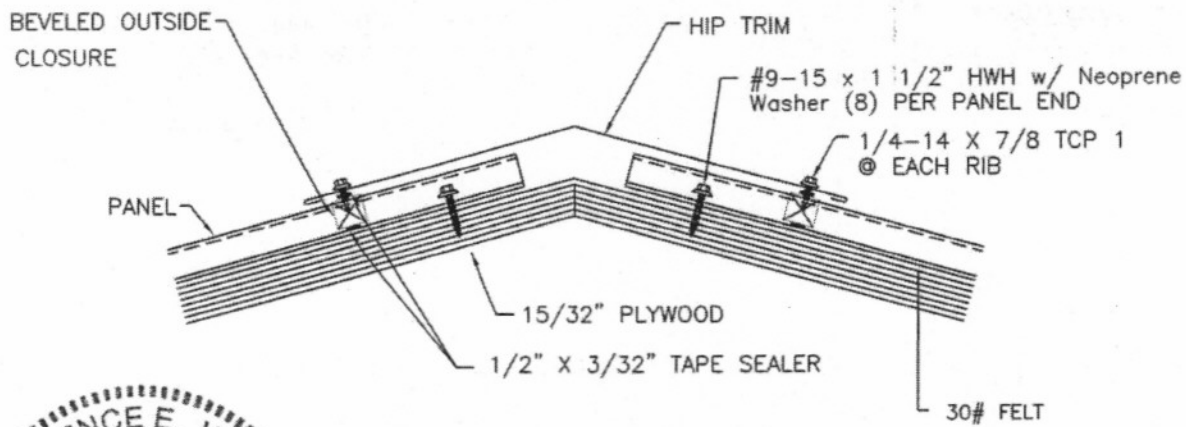
TYPICAL DETAILS HIP
