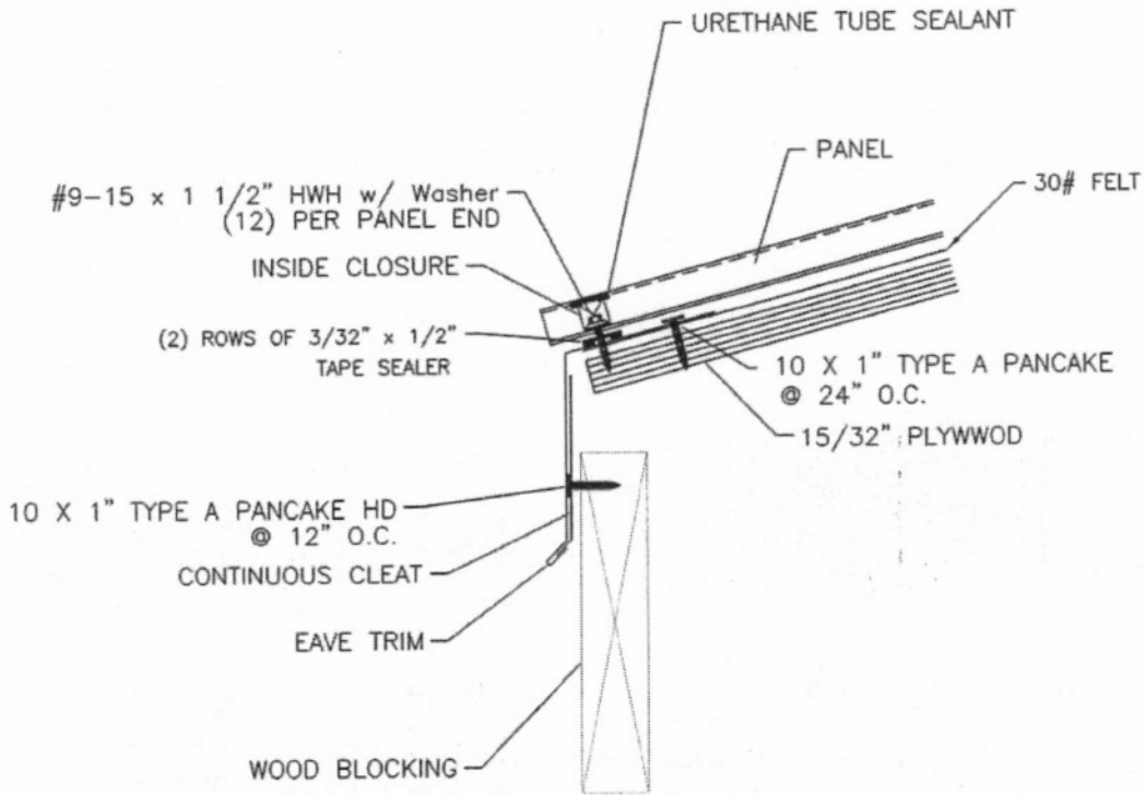
TYPICAL DETAILS EAVE
