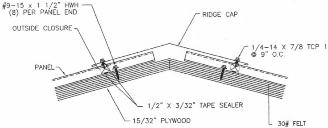
TYPICAL DETAILS RIDGE
